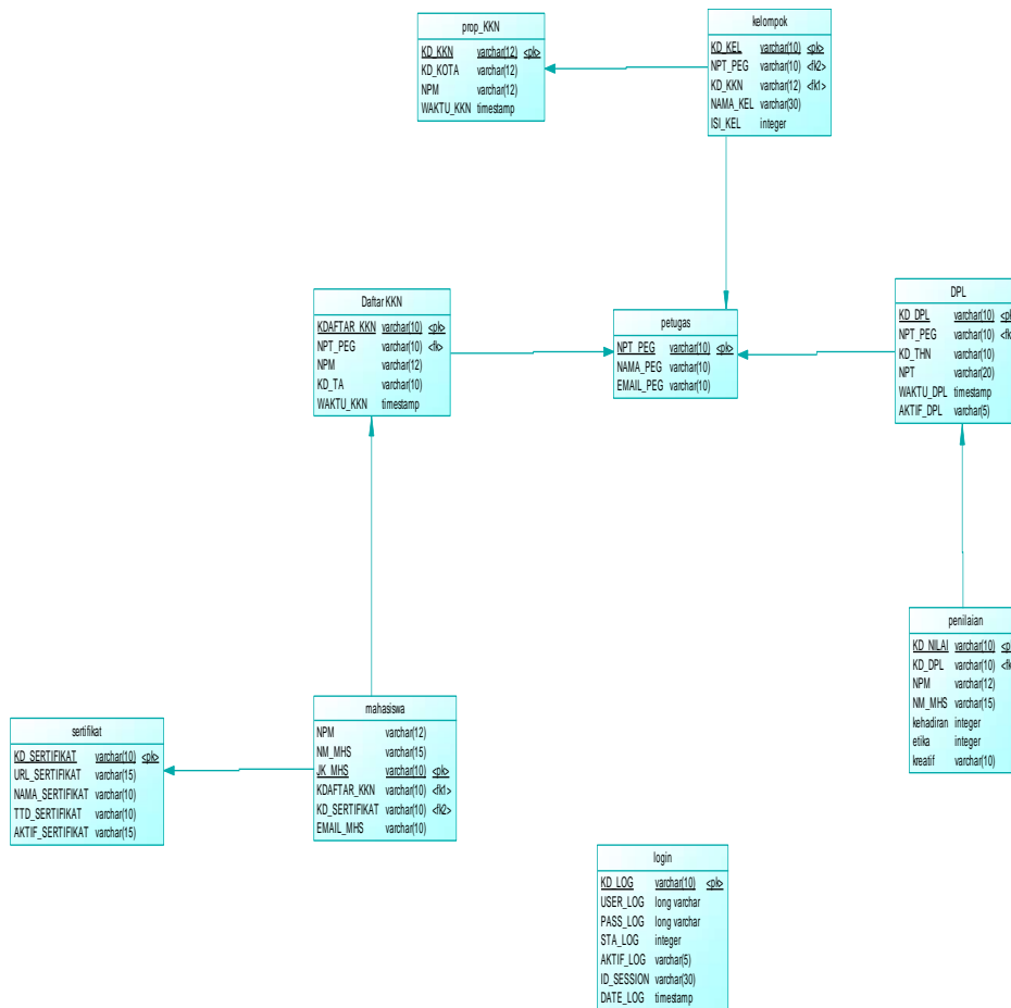
Gambar 4. Physical Data Model
