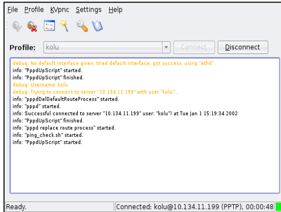
Gambar 8: Connected Client
